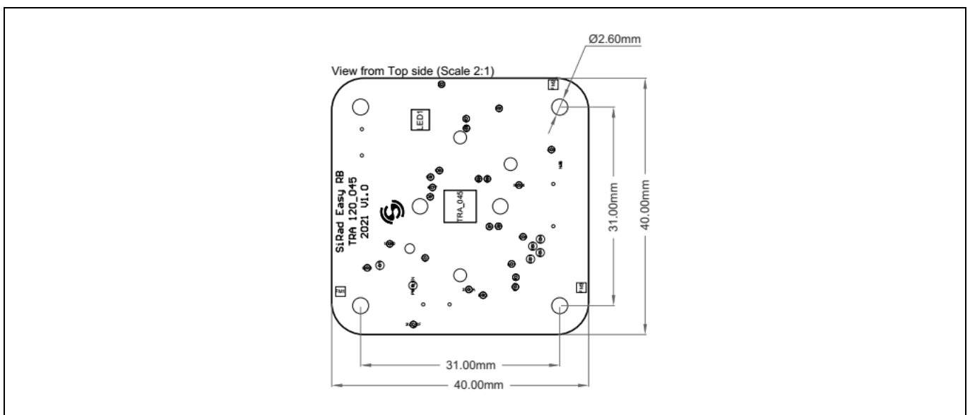
Figure 1 Mechanical Drawing
